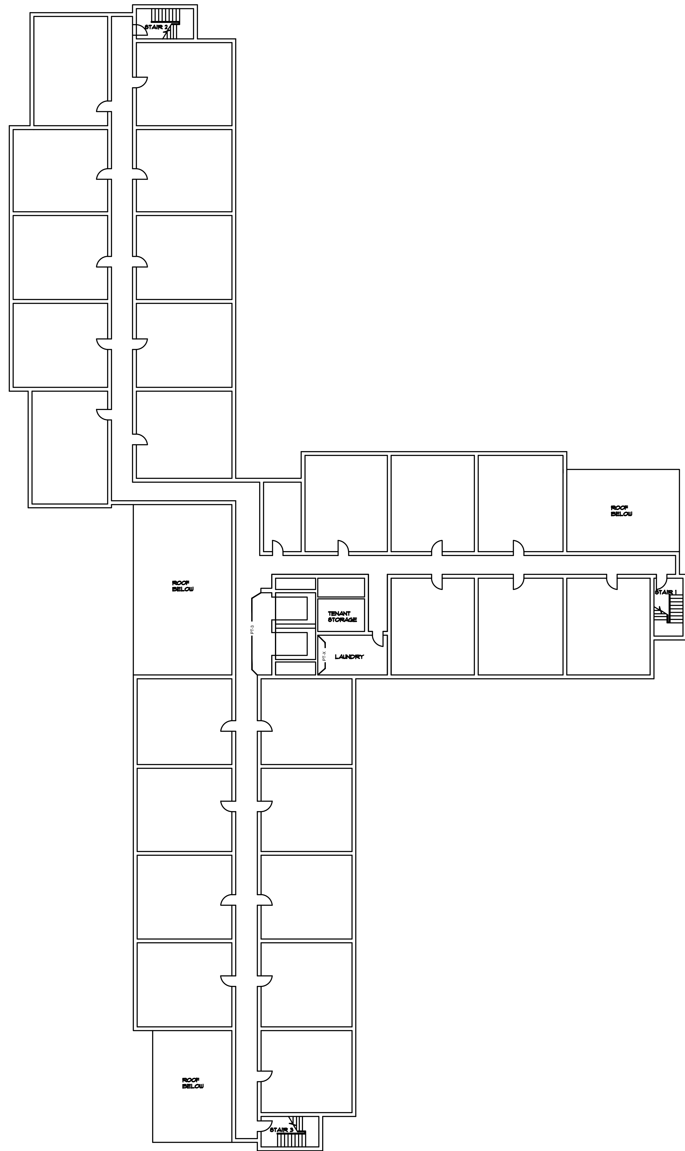
1 SEVENTH FLOOR WALL FINISH PLAN ID. 204 PLAN NORTH
