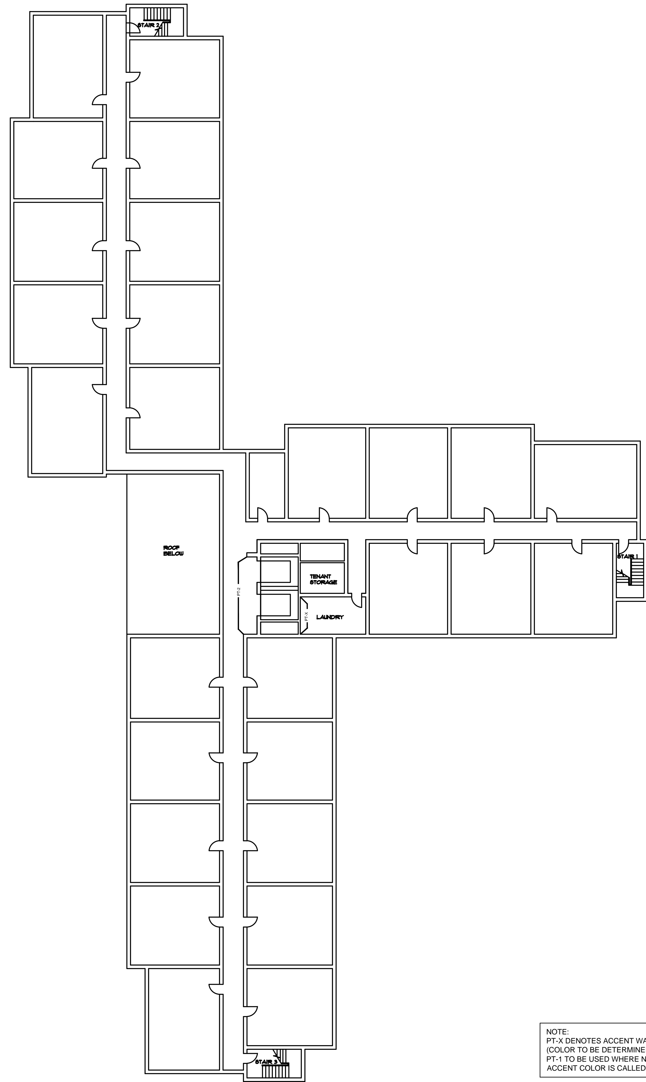
2 SIXTH FLOOR WALL FINISH PLAN ID. 203 PLAN NORTH
